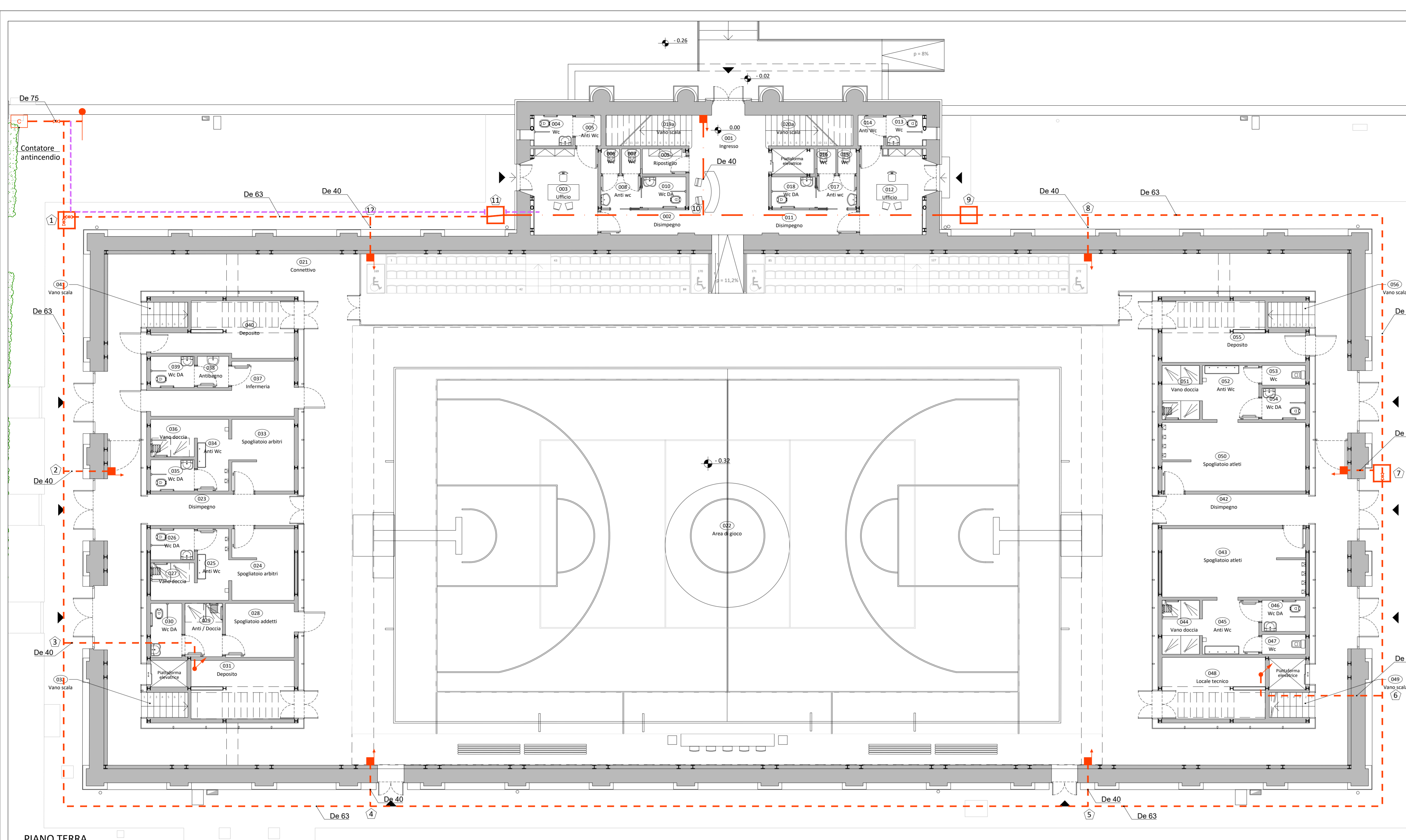
PIANO TERRA
